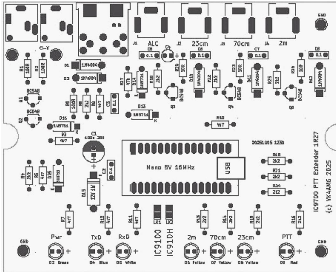
Top side component layout Leaded
